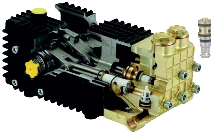
Cut-away pump view
